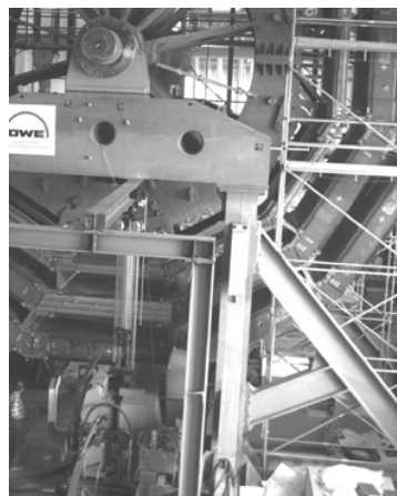
Figure 6 : Barrel Yoke with supporting feet and scaffoldings
