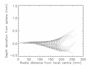
Figure 14: Depth deviation data optimised to a sphere
