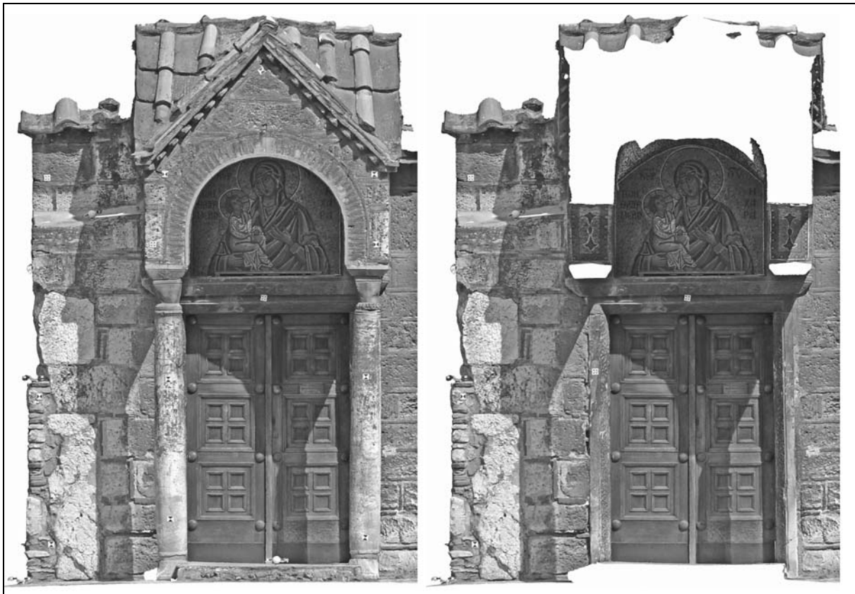
Figure 6. Left: full orthoimage from 7 images. Right: orthoprojection of a model section defined by a maximum Z-value.
