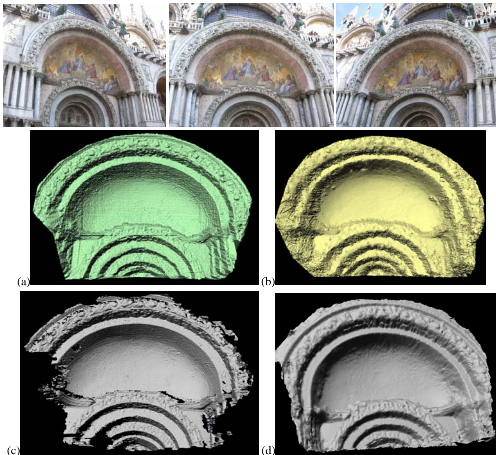
Figure 7: Venice portal, modeled with 3 very convergent images: results from NGATE (a), ATE (b), ARC 3D (c) and SAT-PP (d). ATE presents a quite smooth and noisy surface model compared to the other results. ARC 3D ended with some gaps in the final model. Great experience to correctly tune the different parameters of the tools is really required.
