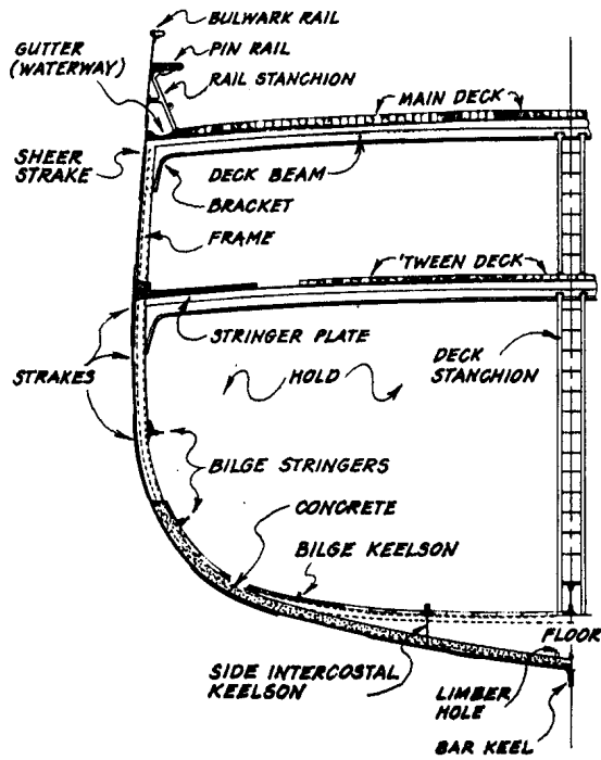
Section through Metal Vessel
