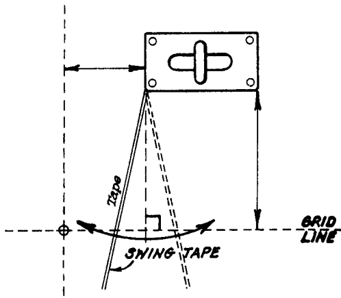
Fig. 4.3.29 Offsets from Grid Lines
