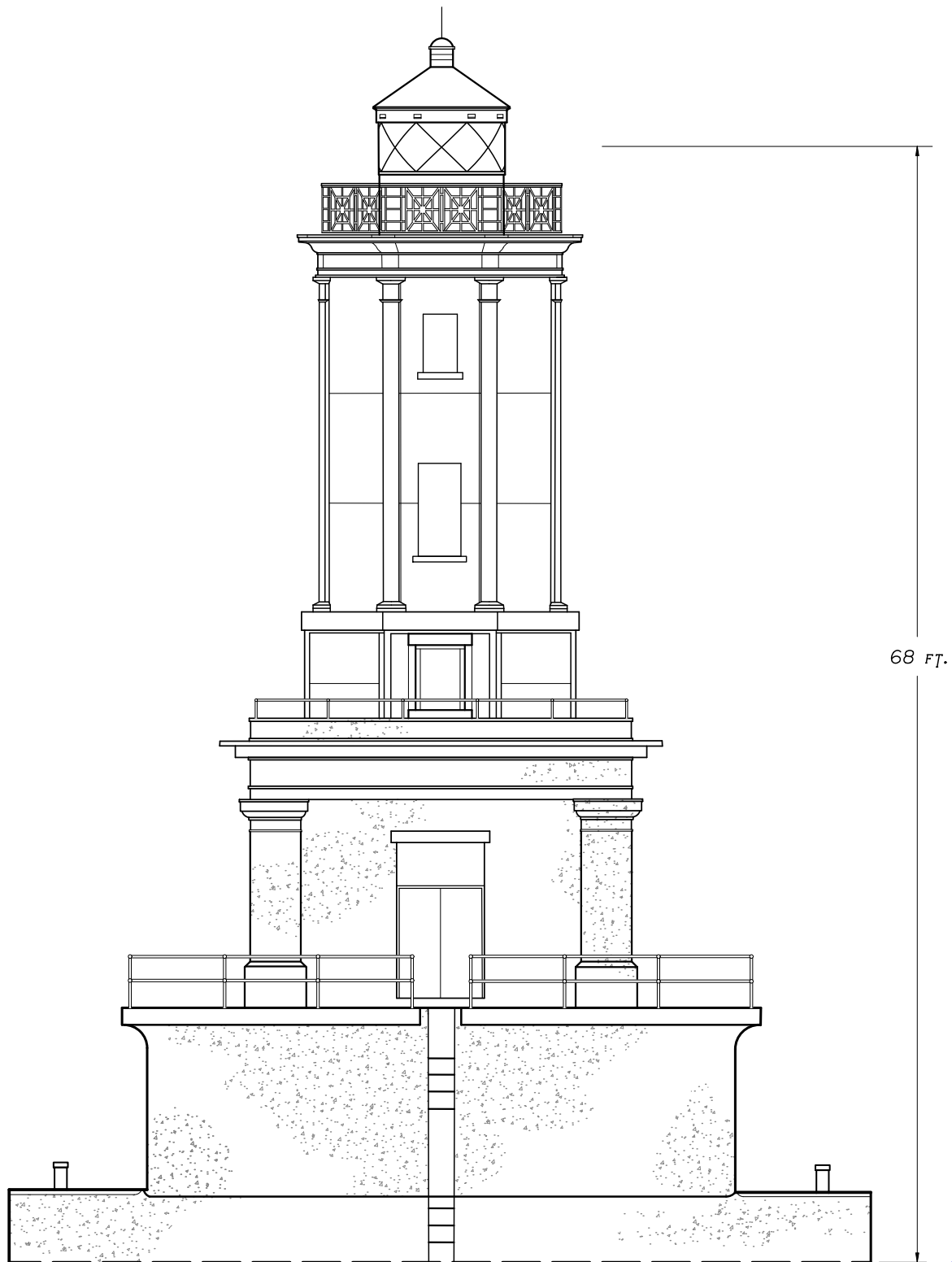
WEST ELEVATION
