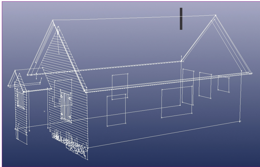
Wire frame model of building surveyed photogrammetrically
