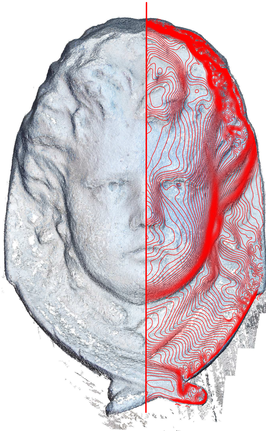
Contour map of architectural detail superimposed on point cloud
